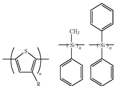
Poly thiohene
