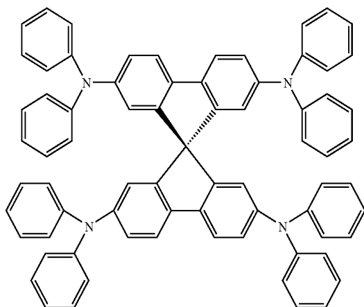
spiro-TPD
